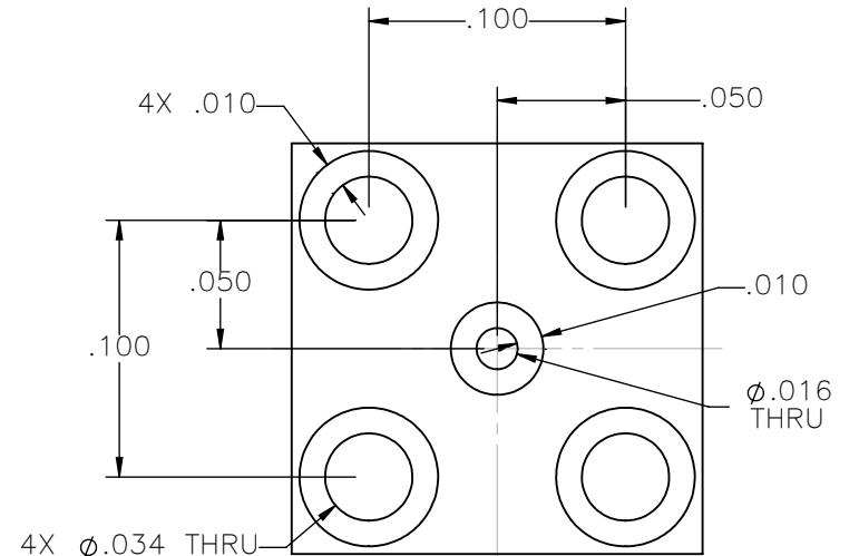
RECOMMENDED PCB LAYOUT 12:1 SCALE
